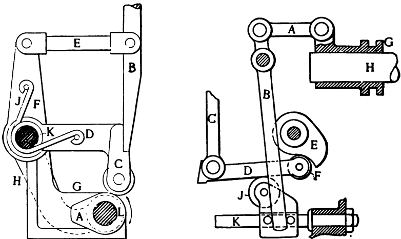
FIG. 214.—Hit and Miss Governor Mechanism of the later Daimler Motors. FIG. 215.—Mechanism of the Peugeot Variable Exhaust Valve Lift.
